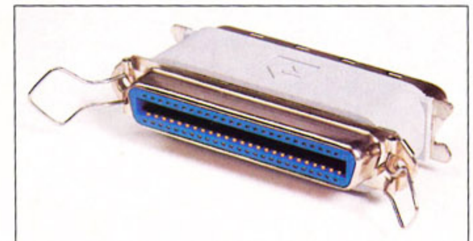
A SCSI terminator is like a SCSI plug with no cabling attached. It simply marks the end of the SCSI chain and 'damps' the electrical signals flying up and down the chain.
