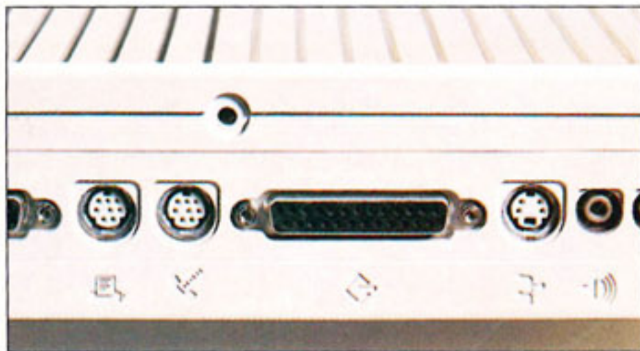
There's a very handy rule of thumb when dealing with Mac connections: if the plug fits, you've probably got the right port. In the case of SCSI, it's the one with the completely unintelligible diamond symbol – so now you know.
